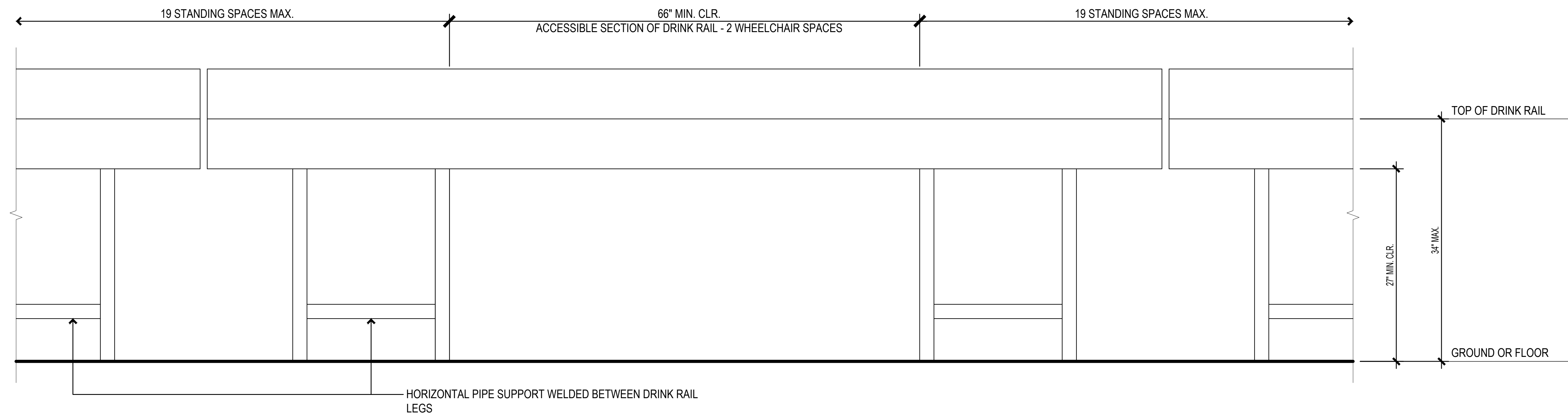
Exhibit F - Drink Rail Detail
